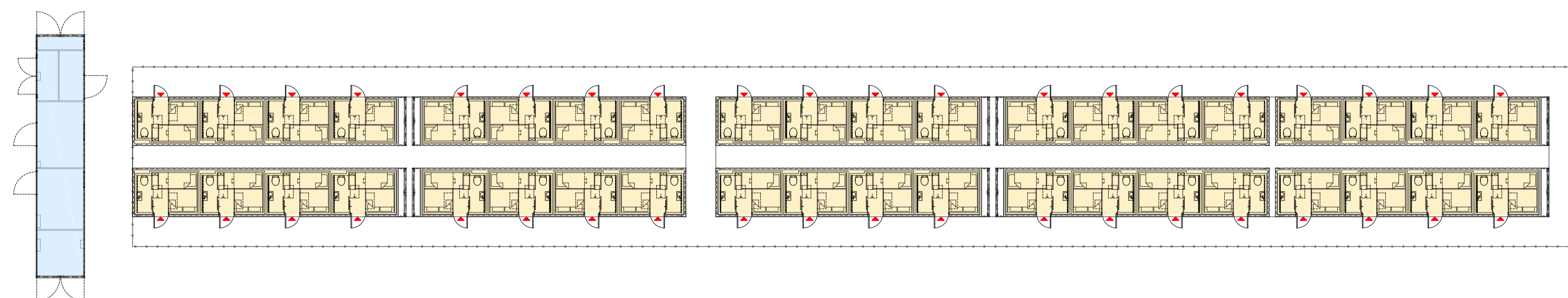
80no. Option - 2 banks of units 1:200
